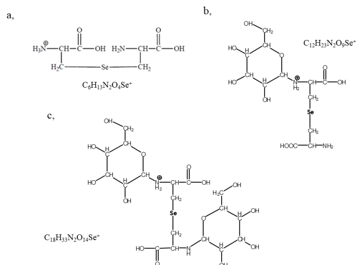
Figure 3. Structures of (a) selenolanthionine, (b) mono- N -glycoside of selenolanthionine, (c) di- N -glycoside of selenolanthionine
