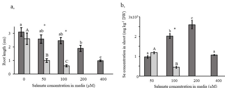
Figure 4. (a) Root length and (b) selenium concentration in shoots of C. violifolia and C. pratensis grown on agar media supplied with different concentrations of \text{Na}_2\text{SeO}_4 . Values shown are the means \pm SEM. Different letters indicate statistically different means among treatments within species ( P < 0.05 ). Asterisks indicate statistically different means between species within treatments ( P < 0.05 ). Note: there was no germination for C. pratensis on 200 and 400 \mu\text{M} Se. In the case of the control treatment, Se concentrations were below the quantification limit.
