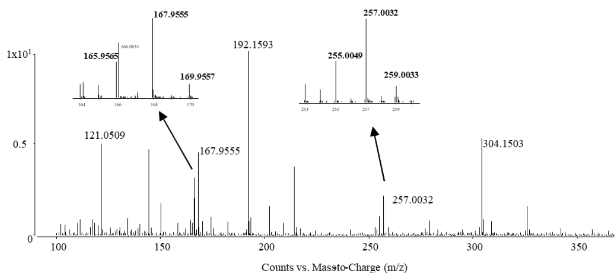
Figure 1. HPLC-ESI-QTOF-MS full scan spectrum recorded at 0.502 min of the most abundant selenium containing fraction of C. violifolia . The spectrum presents the isotopologue patterns of selenolanthionine and its in-source fragment in the insets. Masses highlighted in bold refer to the 78 Se, 80 Se and 82 Se isotopologues. The mass with m/z 166.0835 arrives from an interference on the 78 Se isotopologue of the in-source fragment.
