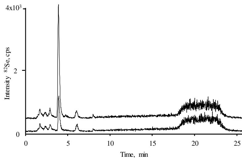
Figure 2. SCX – ICP-MS chromatograms of the C. violifolia water extract (lower chromatogram) and that of the water extract spiked with the synthesised selenolanthionine standard (upper chromatogram).
