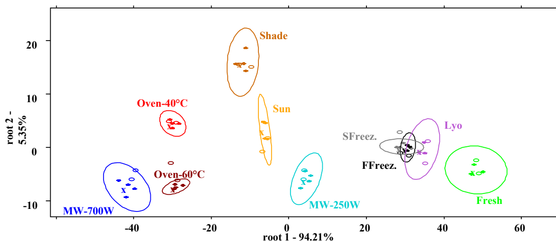
Figure 45. Linear discriminant analysis (LDA) classification model for the grouping of preservation methods based on electronic tongue results applied on Artemisia dracunculus L. 'Artemis'
