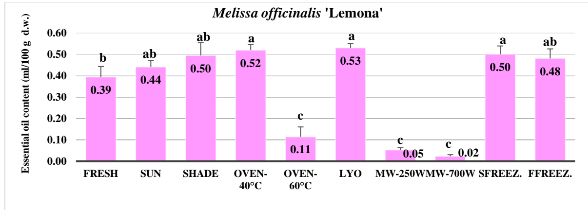
Figure 17. Essential oil content (ml/100 g d.w.) of fresh and preserved leaves of Melissa officinalis L. 'Lemona'
