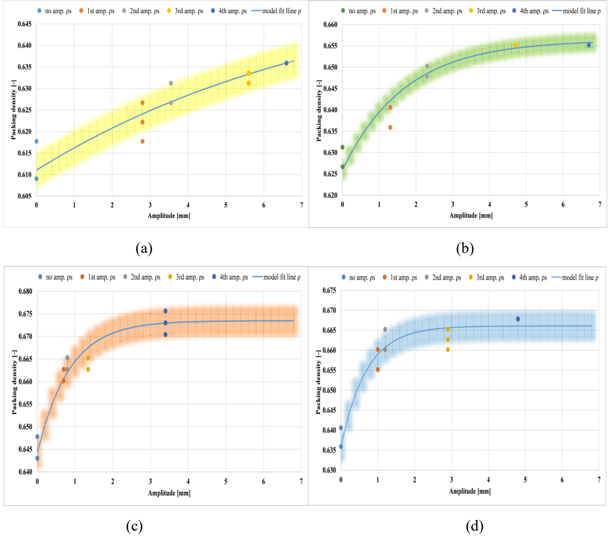
Figure 3.42. The uncertainty of wheat packing density \rho vs the vibration amplitude A for four different normal stresses
