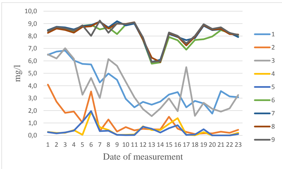
Figure 5: Time evolution of dissolved oxygen content of the treatments 1 control; 2 mechanical mixing; 3 sodium percarbonate; 4 bacterium product; 5 sodium percarbonate + bacterium product; 6 aeration; 7 aeration + sodium percarbonate; 8 aeration + bacterium product; 9 aeration + sodium percarbonate + bacterium product
