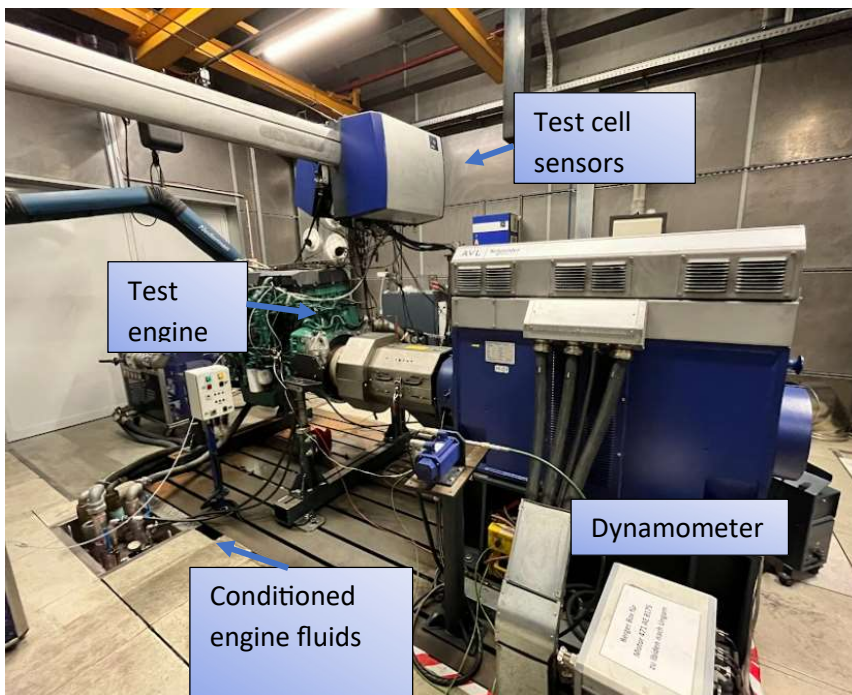
Figure 1. Engine dynamometer test cell at Ibiden Hungary Ltd.'s facility (Source: Norbert Biró)
