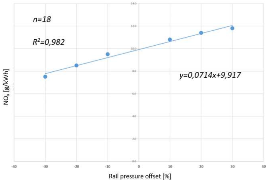
Figure 12 \text{NO}_x as a function of changes in common rail pressure during the WHSC cycle. (Source: Norbert Bíró)
