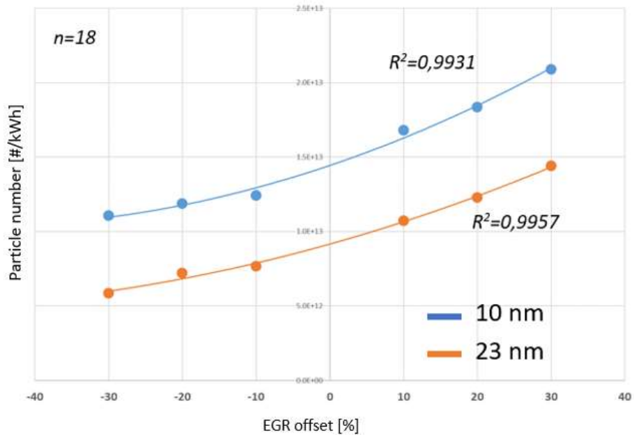
Figure 10 Particle number of 10 and 23 nm as a function of changes in exhaust gas recirculation during the WHSC cycle. (Source: Norbert Bíró)
