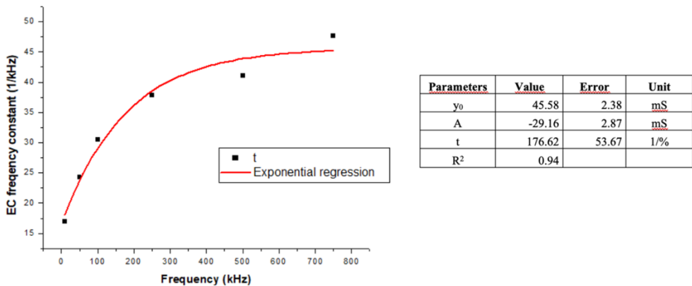
Fig. 14 Values of the frequency constant as a function of the measurement frequencies and fitting of the exponential function
