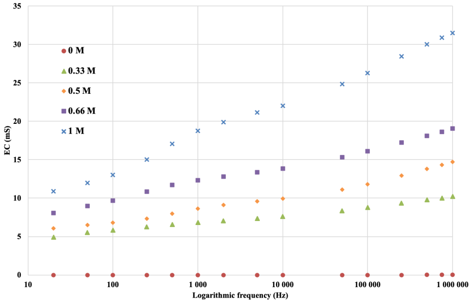
Fig. 6 EC as a function of logarithmic measurement frequency for soil solutions soaked with different concentrations of KCl
