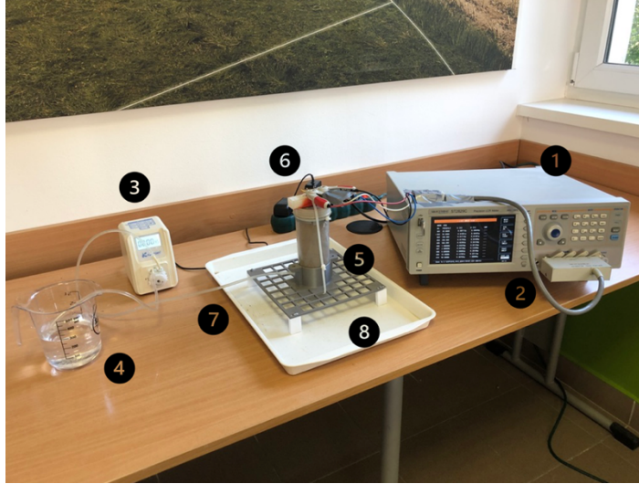
Fig. 1 The measuring circuit for experiments with soil paste
