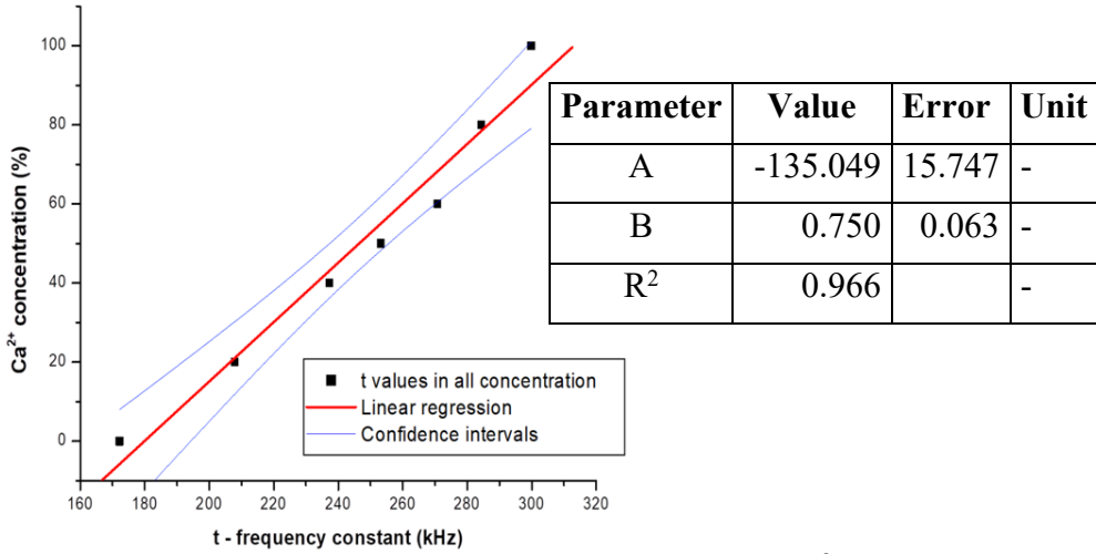
Fig. 16 The frequency constant ( t ) is a function of the \text{Ca}^{2+} concentration of the two-component solution
