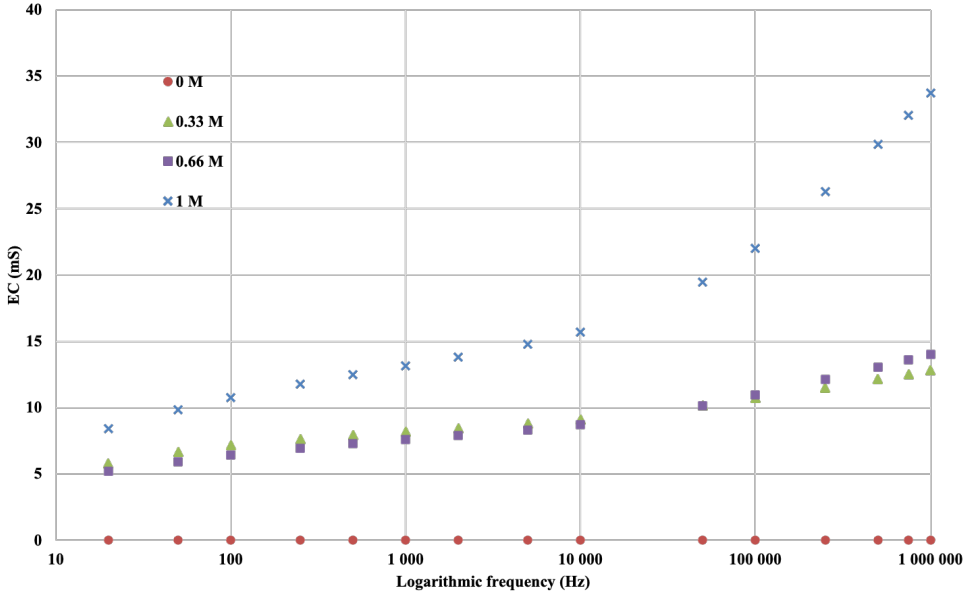
Fig. 8 EC as a function of logarithmic measurement frequency for soil solutions soaked with different concentrations of CaCl2
