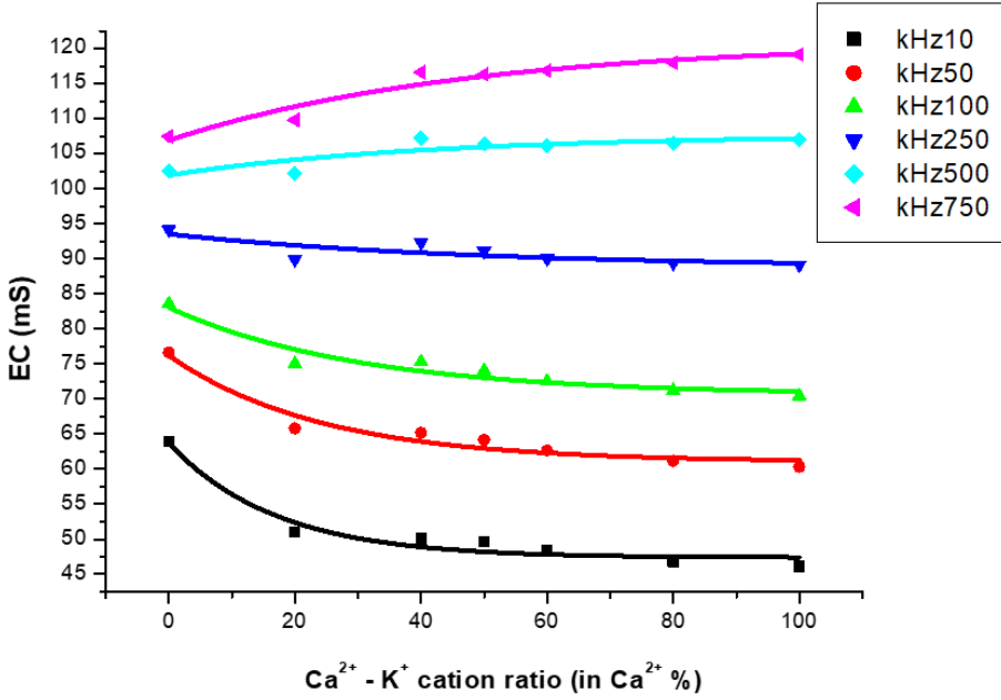
Fig. 11 Comparison of measurements and function matching
