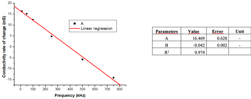
Fig. 13 Values of the rate of change as a function of measurement frequencies and linear function fitting
