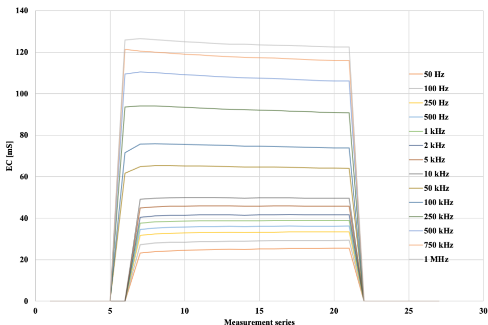
Fig. 5 Diagram of EC value per measurement sequence of 50 % KCl – 50 % CaCl 2 mixture solution
