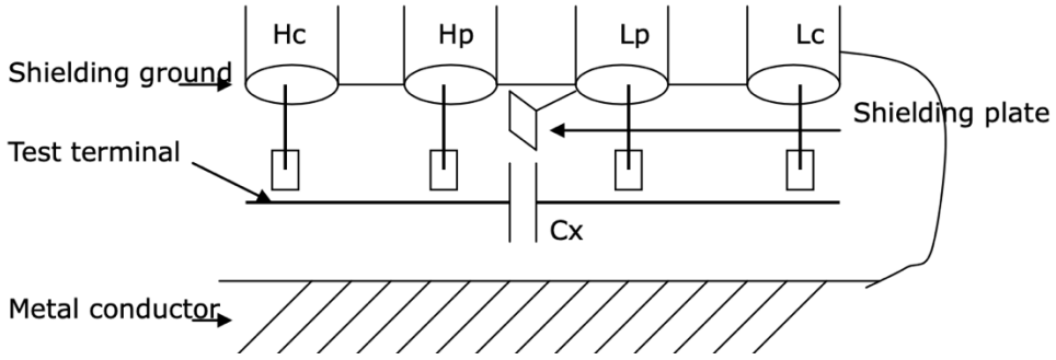
Fig. 3 Method of measurement to eliminate interference
