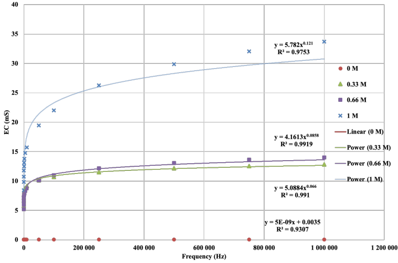
Fig. 9 EC saturation curve plotted on a natural scale for soil solutions with different \text{Ca}^{2+} concentrations
