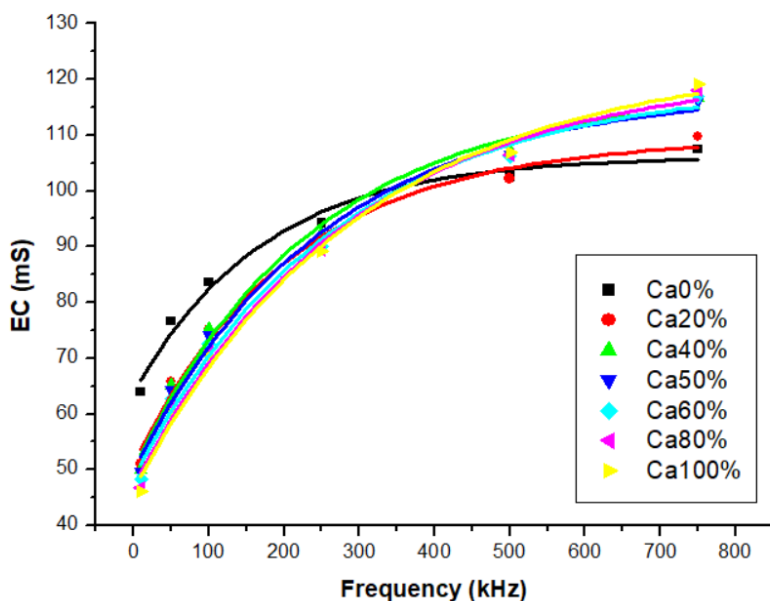
Fig. 15 Comparison of measurements of different two-component mixtures as a function of frequency
