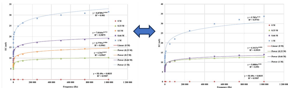
Fig. 18 The reference functions for potassium ( K^+ ) and calcium ( Ca^{2+} ) differ
