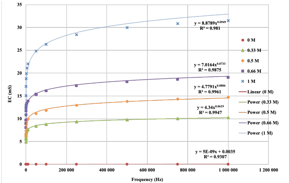
Fig. 7 EC saturation curve for soil solutions of different K^+ concentrations
