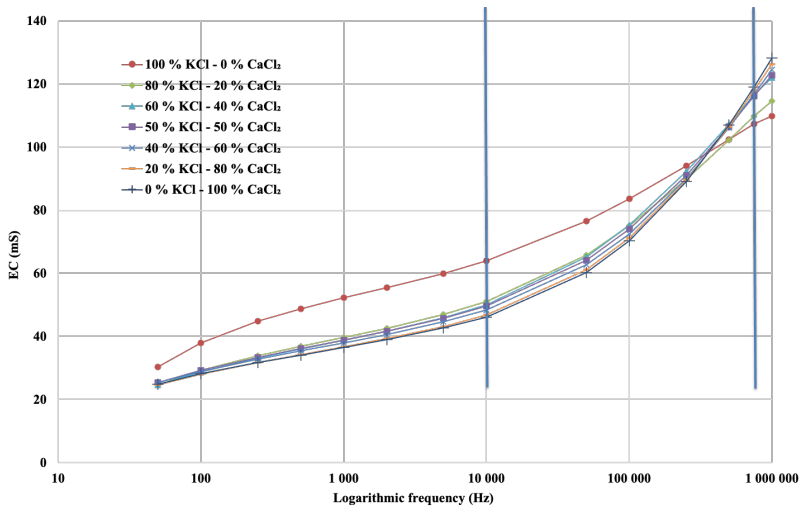
Fig. 10 Comparison of EC measurements of different mixtures
