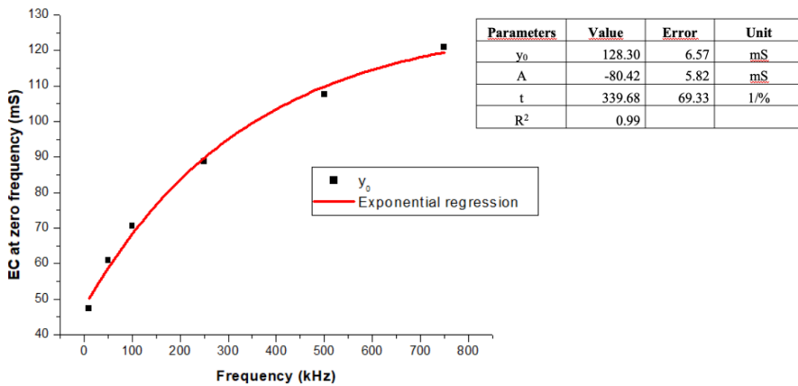
Fig. 12 Conductivity extrapolated to zero frequency as a function of measurement frequencies and matching of exponential function
