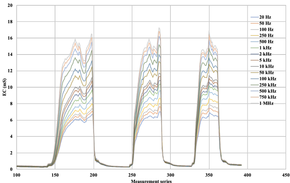
Fig. 4 Diagram of EC value per soil solution measurement sequence
