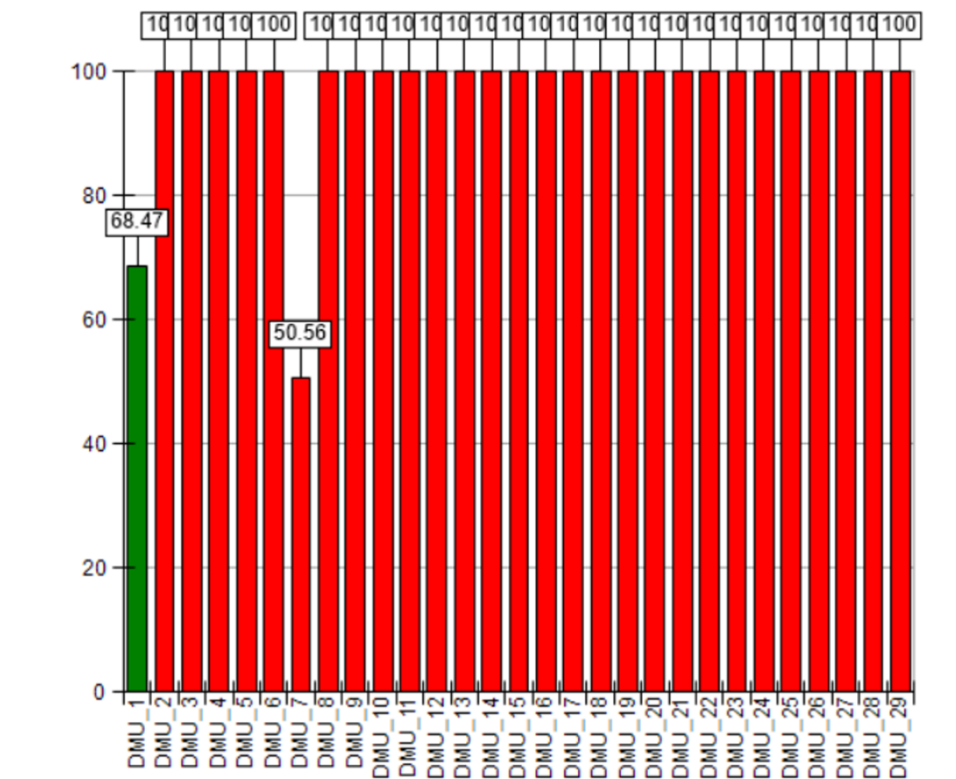
Figure 17. DEA Analysis with Variable Returns to Scale (VRS-Input) Utilizing Urban Input Variables Group. Source: Researcher, 2023.
