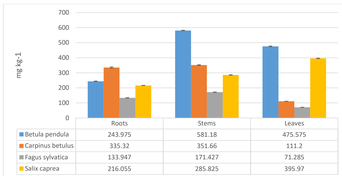
Figure 7. Concentration levels ( \text{mg kg}^{-1} ) of Zn in roots, stem and leaves of tree species growing in mined spoil soils in Mátraszentimre, Máttra Mountains, Hungary.
