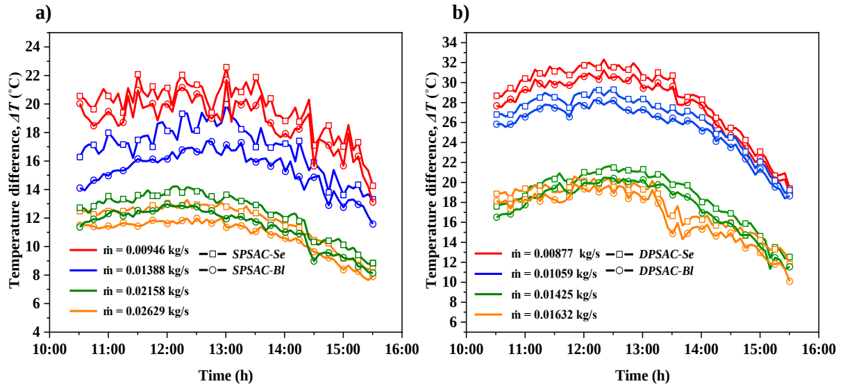
Fig. 4.29. The temperature difference across the collectors versus time for (a) SPSAC and (b) DPSAC
