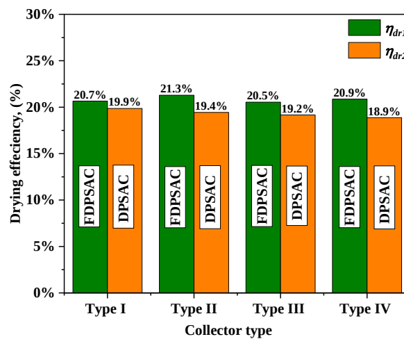
Fig. 4.56. The drying efficiency using proposed configurations
