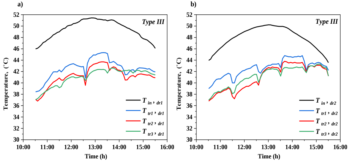
Fig. 4.49. Temperature variation of the drying chambers using: a) Type III FDPSAC, b) smooth DPSAC
