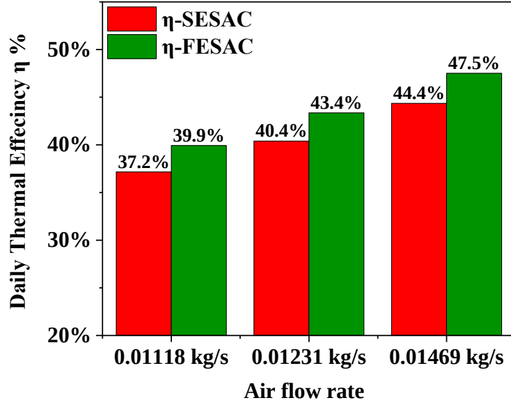
Fig. 4.7. The daily thermal efficiency versus airflow rate
