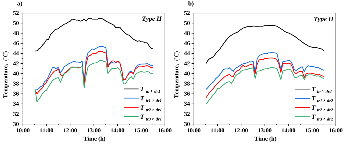
Fig. 4.48. Temperature variation of the drying chambers using: a) Type II FDPSAC, b) smooth DPSAC
