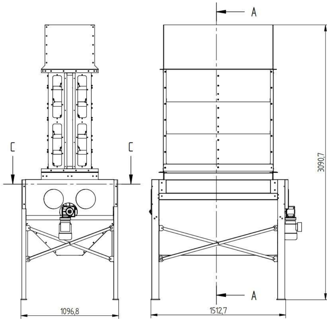
Figure 2.2.: The structure and main dimensions of the model dryer
