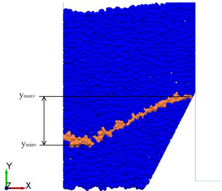
Figure 2.7.: Determination of flow unevenness based on particle displacement
