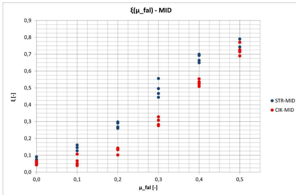
Figure 2.12.: The \xi values determined for the marked bands in the case of straight (STR) and cycloid (CIK) lamellae as a function of the grain-wall friction coefficient
