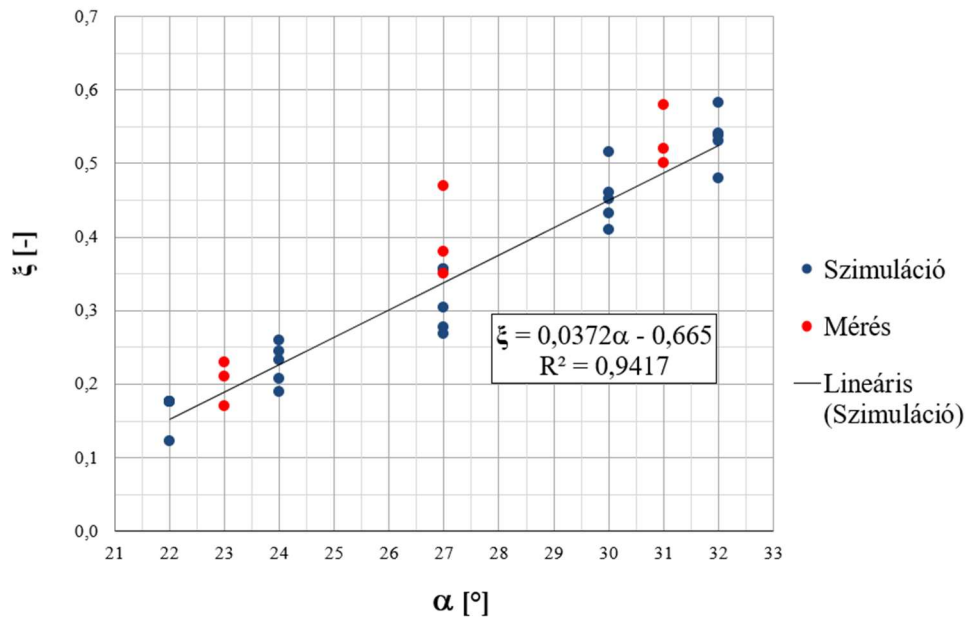
Figure 2.8.: Comparison of the measured and numerically determined unevenness factor values
