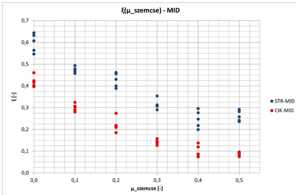
Figure 2.11.: The \xi values determined for the marked bands in the case of straight (STR) and cycloid (CIK) lamellae as a function of the grain-grain friction coefficient
