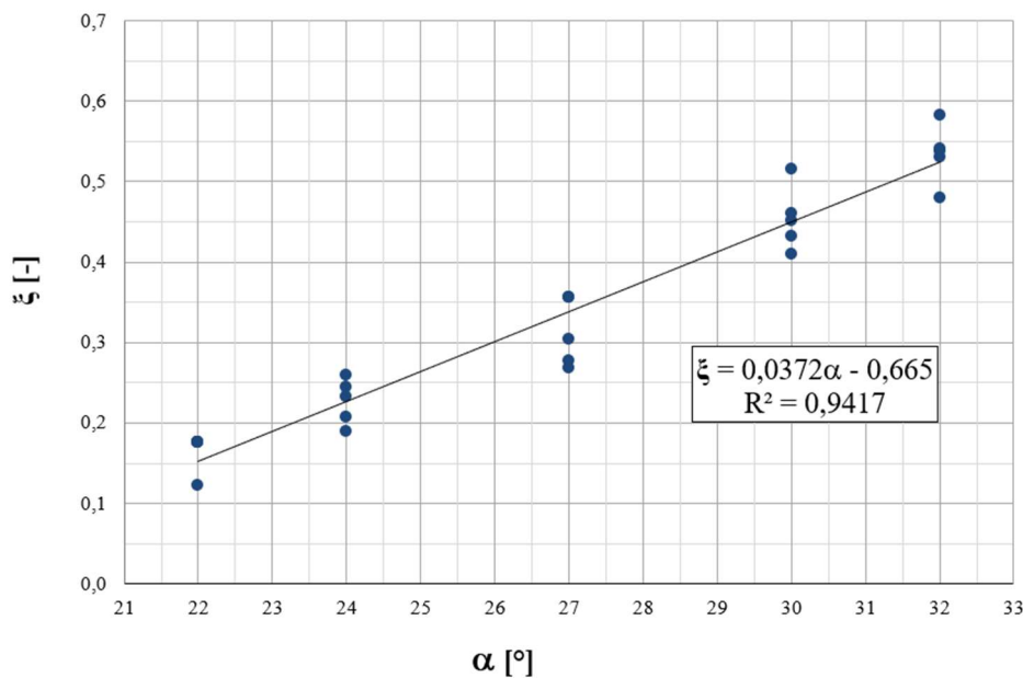
Figure 3.3.: Material flow unevenness as a function of the lamella inclination angle
