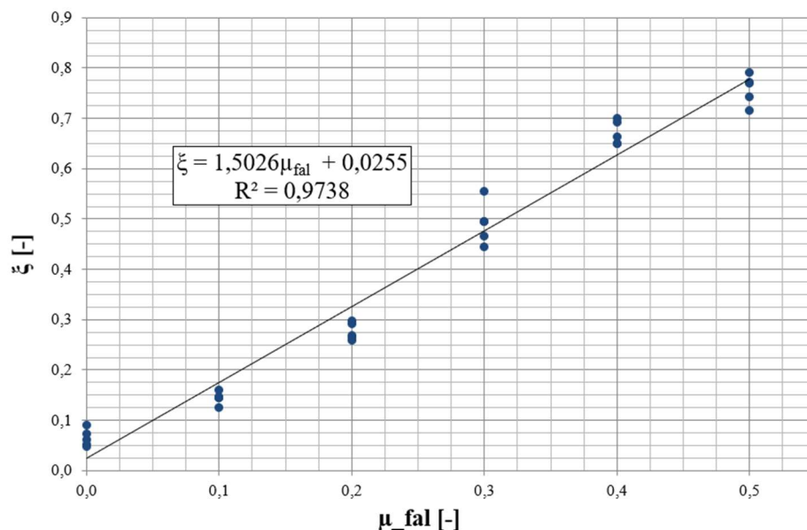
Figure 3.1.: Material flow unevenness as a function of the grain-wall friction coefficient for a 27^\circ lamella inclination angle
