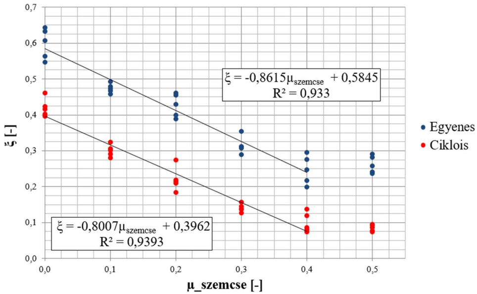
Figure 3.5.: Material flow unevenness as a function of the grain-grain friction coefficient for straight (27°) and cycloid lamellae
