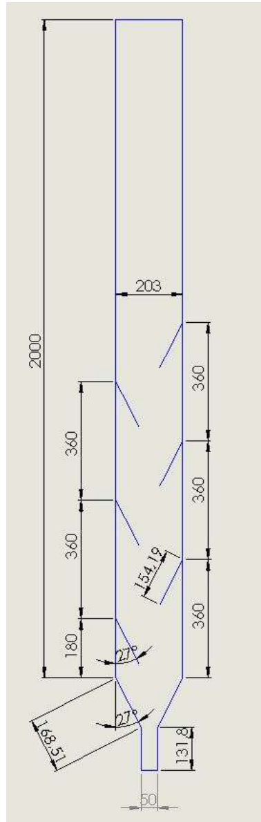
Figure 2.5.: The geometry in the numerical model
