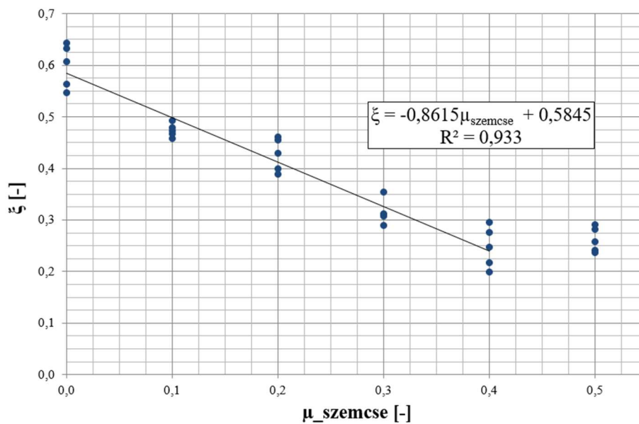
Figure 3.2.: Material flow unevenness as a function of the grain-grain friction coefficient for a 27° lamella inclination angle
