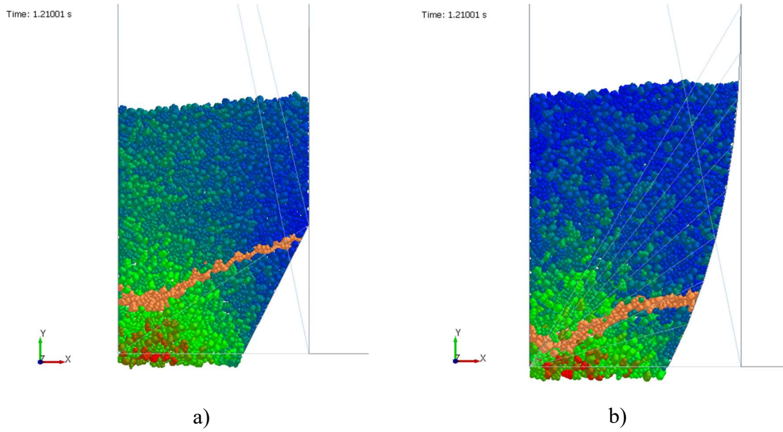
Figure 2.10.: The shape of the centrally positioned marked bands after \Delta t = 0.21 s for a) straight and b) cycloid-shaped lamella
