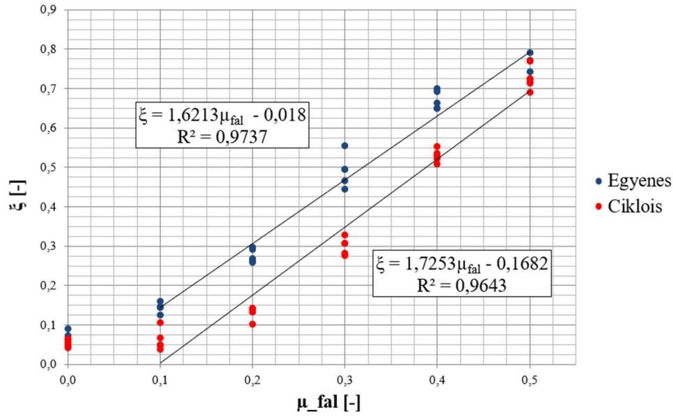
Figure 3.4.: Material flow unevenness as a function of the grain-wall friction coefficient for straight (27°) and cycloid lamellae
