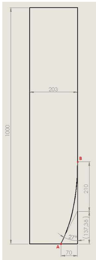
Figure 2.9.: Module geometry for the comparison of straight and cycloid-shaped lamellae
