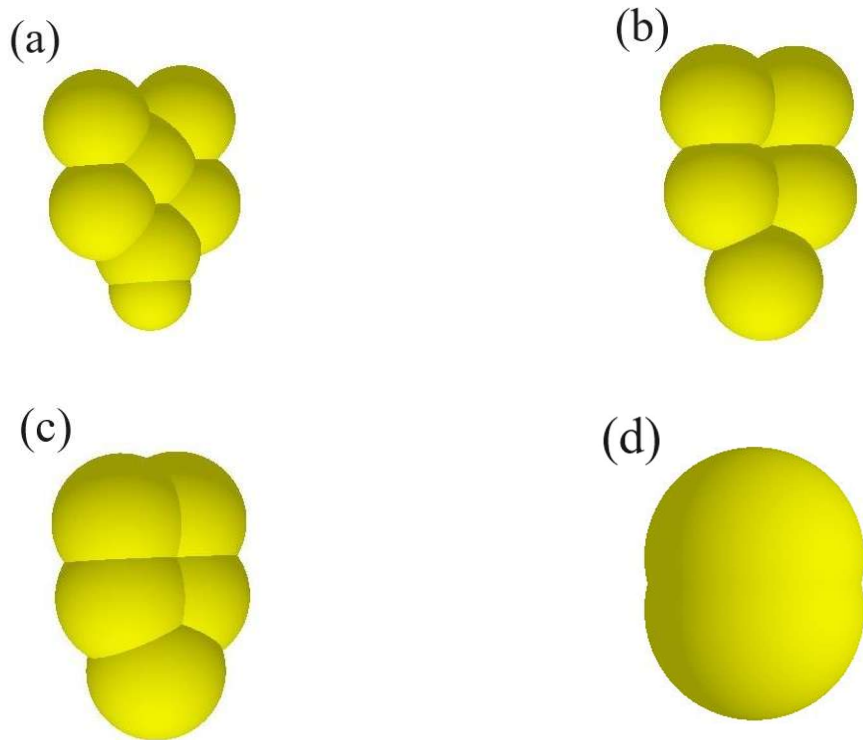
Figure 2.4.: Particle shapes used in the discrete element simulations: (a) flat, (b) elongated, (c) angular, (d) round
