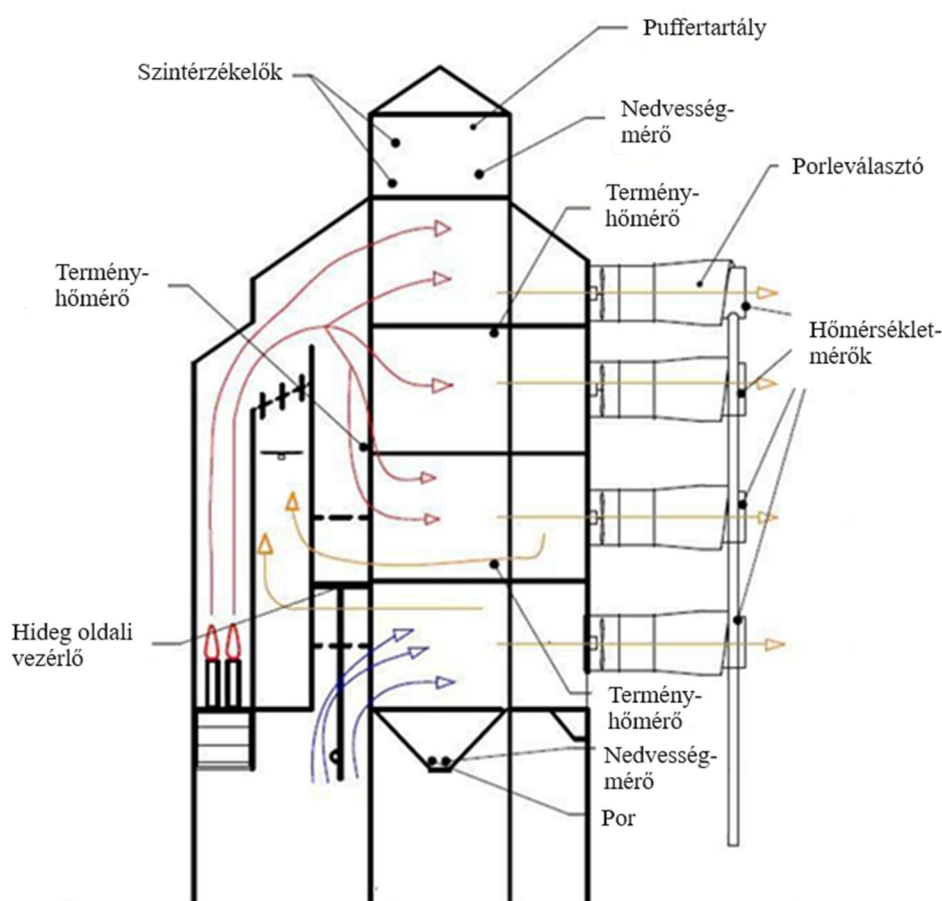
Figure 2.1.: Main components of the industrial dryer
