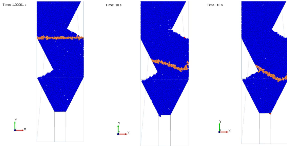
Figure 2.6.: The position of the marked bands at the initial time (1 s), and after 10 s and 13 s for a 27° lamella inclination angle
