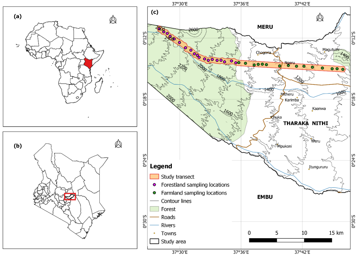
Figure 1: Map of the study area showing (a) The location of Kenya in Africa, (b) The location of the study area in Kenya, (c) The study transect and sampling locations on the eastern slopes of Mount Kenya. (Source: author)
