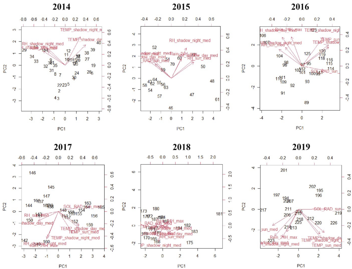
Figure 5: Results of PCA among different weather parameters.
