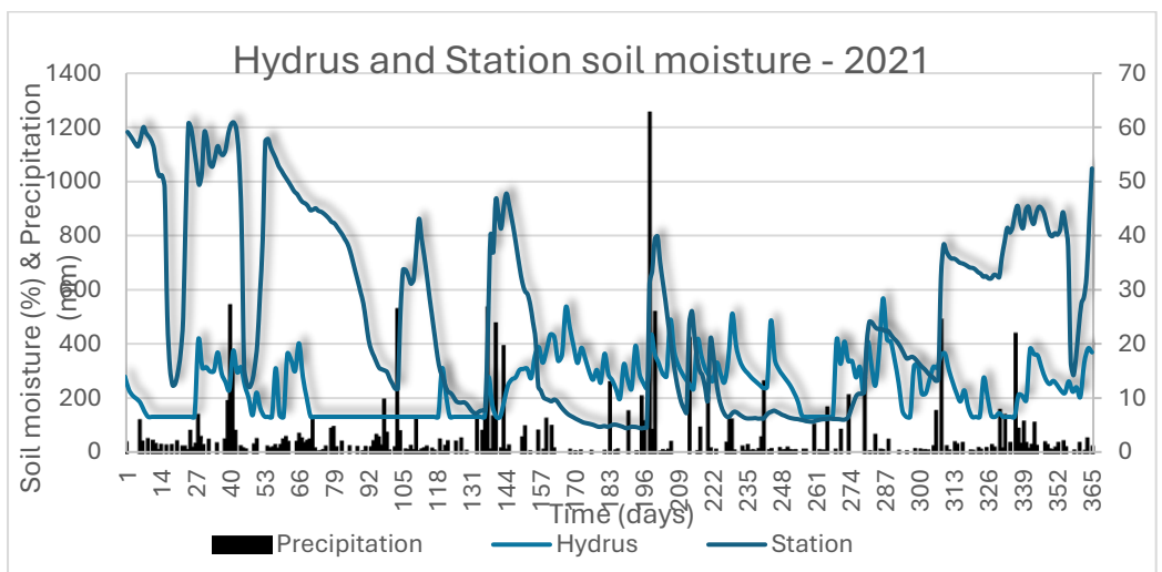
Figure 13 - Hydrus and Research station Soil moisture – 2021
