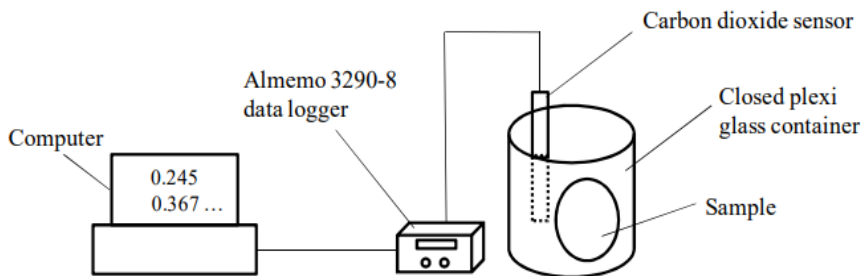
Figure 5: Schematic diagram of respiration measurement
