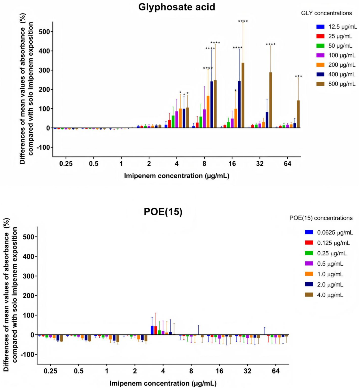
Figure 13. Differences in averaged absorbance of the five P. aeruginosa strains (ATCC 27853, ATCC 10145, ATCC 15442, HF234, P66) during co-exposure to the combination of test materials (glyphosate, POE(15), GBHs) and imipenem compared to solo imipenem exposition with the same concentration (expressed in %). Statistical analysis: Two-way ANOVA and Dunnett’s multiple comparisons tests. *, **, *** and **** are significantly different from solo imipenem values ( p < 0.0332 , p < 0.0021 , p < 0.0002 and p < 0.0001 , respectively).
