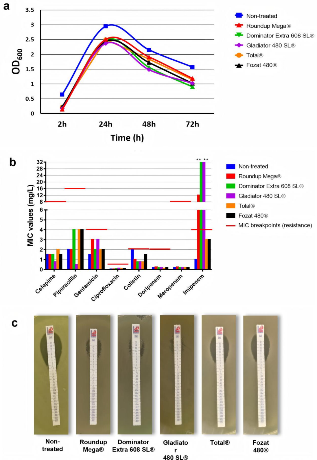
Figure 11. Pre-exposure of P. aeruginosa HF234 using 0.5 v/v% GBHs (averaged values obtained from three technical replicates). (a) The optical density ( OD_{600} ) of broth cultures which was treated with GBHs for 72 h. (b) MIC values of HF234 cultures after 72 h pre-exposure, plated on GBH-free agar plates. (c) Inhibition zones of HF234 cultures after 72 h GBH pre-exposure, plated on GBH-free plates. * and ** mean significant differences compared to the non-treated strain ( p=0.0332 - 0.0023 ). Figure was created by Jiang D. and Kaszab E. (HÁHN et al., 2022)
