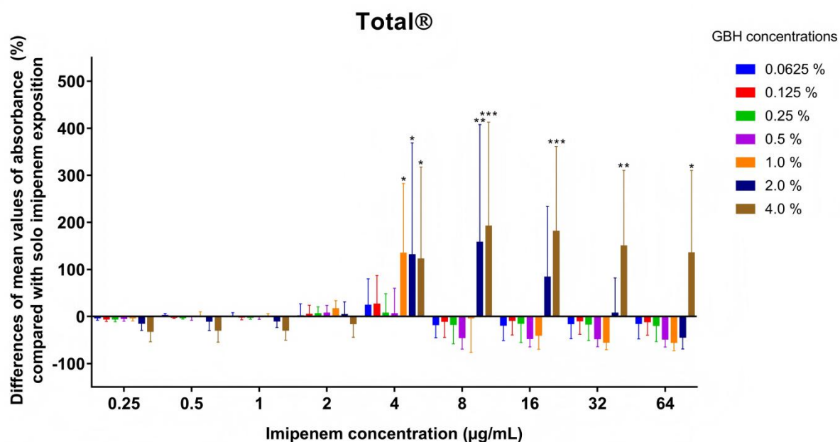
Figure 13. (cont.) Differences in averaged absorbance of the five P. aeruginosa strains (ATCC 27853, ATCC 10145, ATCC 15442, HF234, P66) during co-exposure to the combination of test materials (glyphosate, POE(15), GBHs) and imipenem compared to solo imipenem exposure with the same concentration (expressed in %).
