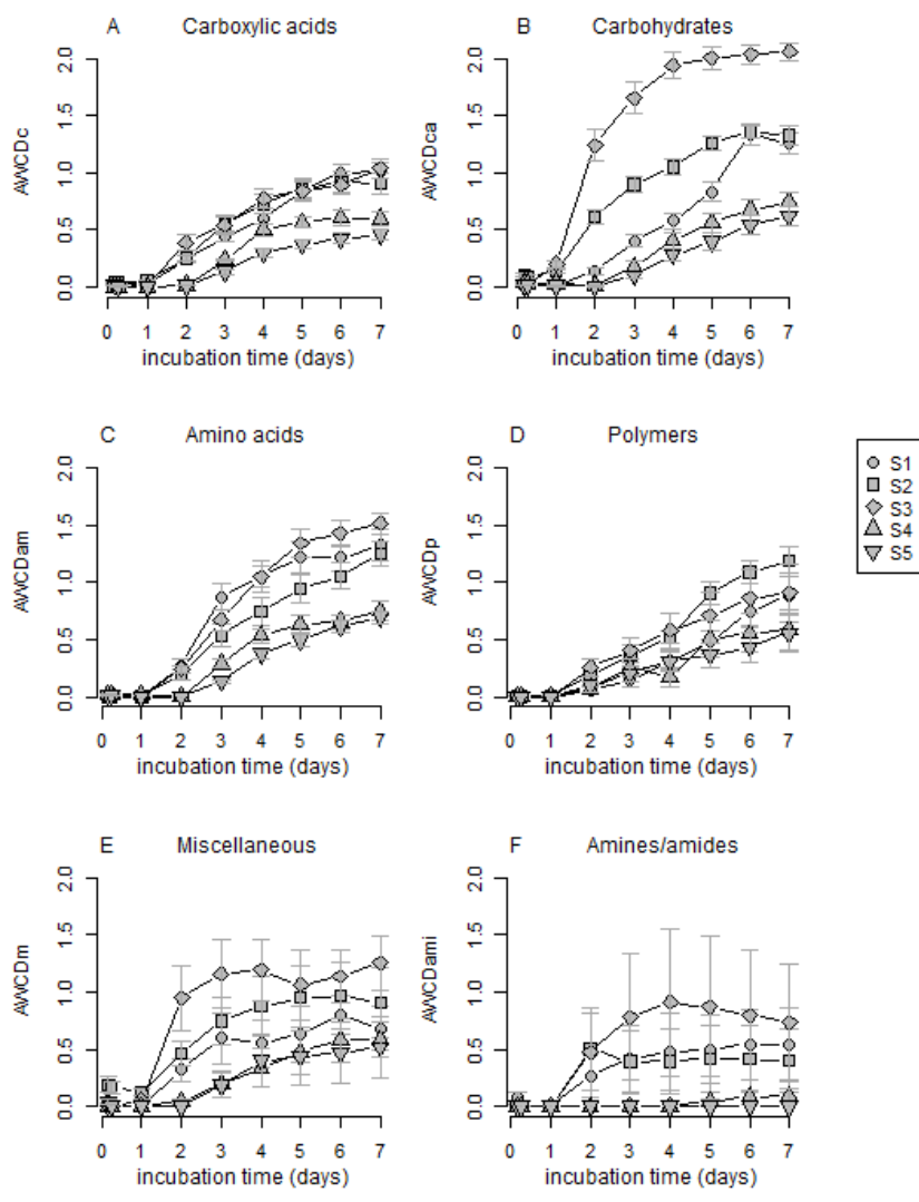
Figure 17. The Average well color development of six types of carbon sources in five soil microbial communities, including carboxylic acids (A), carbohydrates (B), amino acids (C), polymers (D), miscellaneous (E), and amines/amides (F).
