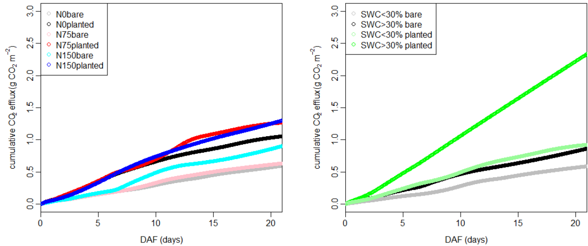
Figure 27. Cumulative CO 2 efflux (g CO 2 m -2 ) courses across the 3 weeks long laboratory study period. CO 2 effluxes are separated by N treatments (left panel, 0, 75 and 150 kg N ha -1 ) and by soil water content (right panel, >30% and <30%) in bare and planted soil.
