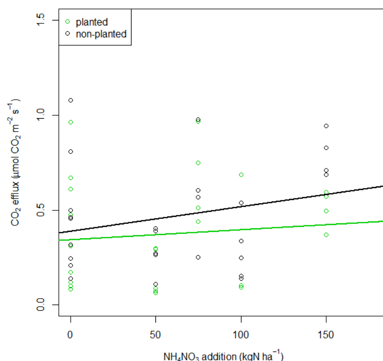
Figure 26. The CO 2 efflux ( \mu\text{mol CO}_2 \text{ m}^{-2} \text{ s}^{-1} ) in planted and non-planted (bare soil) under different NH 4 NO 3 treatments during long laboratory study period
