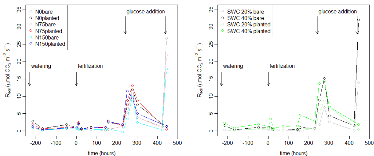
Figure 28. The CO 2 efflux ( \mu\text{mol CO}_2 \text{ m}^{-2} \text{ s}^{-1} ) dynamic during 4 weeks long laboratory study period. CO 2 effluxes are separated by N fertilization (left panel, 0, 75 and 150 kg N ha -1 ) and by soil water content (right panel, 20% and 40%), addition of glucose in the 251 h in bare and planted soil and at 445 h in bare soil.
